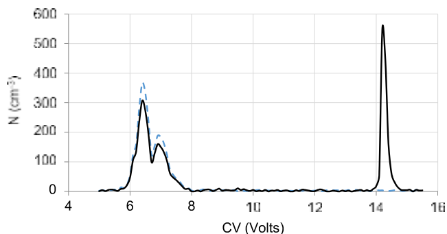
Fig. 4. IIT counts vs. compensation voltage of the ion filter. Clean air containing traces of acetone was introduced into the set-up according to Fig. 2c. The background signal from the clean air is indicated with a dashed line, while the signal from air with acetone is shown with solid line.
