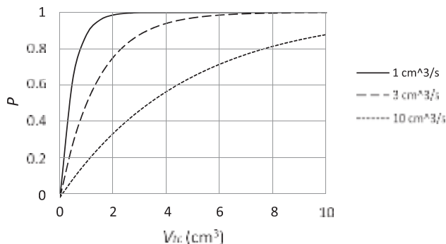
Fig. 1. Charging probability ( P ) of 300 nm spherical tags density 1200 \text{ kg/m}^3 vs. volume of the tagging chamber ( V_{tc} ) at various flow rates by \text{N}^+ ions.
