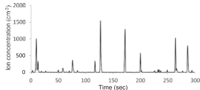
Fig. 3. An IIT counts vs. time for a stainless steel external chamber of 80 \text{ cm}^3 internal volume.
