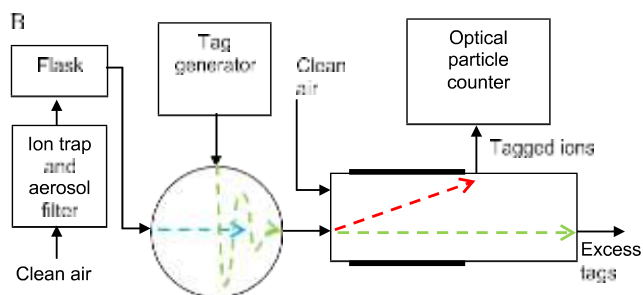
Fig. 2b. Schematic of the set-up with an ion trap and a flask. The rest is the same as in Fig. 2a.
