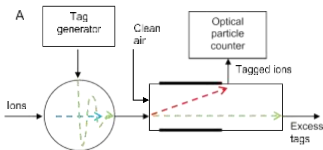
Fig. 2a. Schematic of the ion counting set-up. The tagging object trajectories are shown with dashed green lines. The tagging chamber is shown with a circle. The blue dashed line schematically shows ion trajectories in the tagging chamber. The red dashed line indicates the direction of the tagged ions, and the green horizontal line shows trajectories of neutral tags in the extraction chamber (two bold horizontal lines show electrodes in the extraction chamber). (For interpretation of the references to colour in this figure legend, the reader is referred to the web version of this article.)
