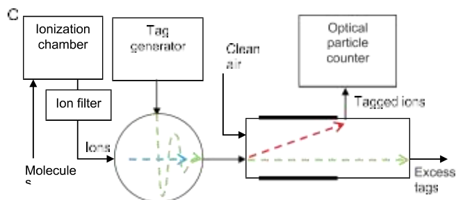
Fig. 2c. Schematic of the molecular counting set-up with an ionization chamber and an ion filter. The rest is the same as in Fig. 2a.
